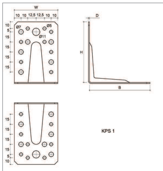
Figure 12 Type KPS 1
