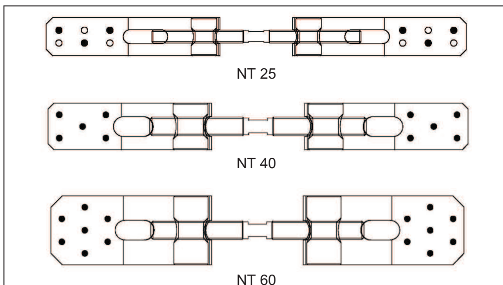
Figure 90 Type NT
