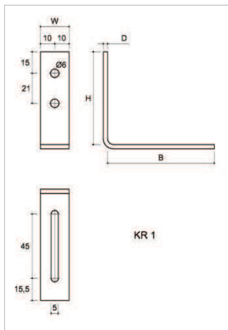
Figure 30 Type KR 1
