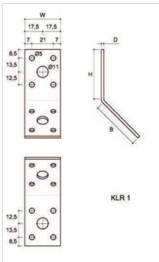
Figure 4 Type KLR 1
