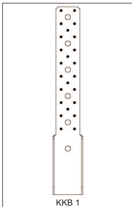
Figure 91 Type KKB
