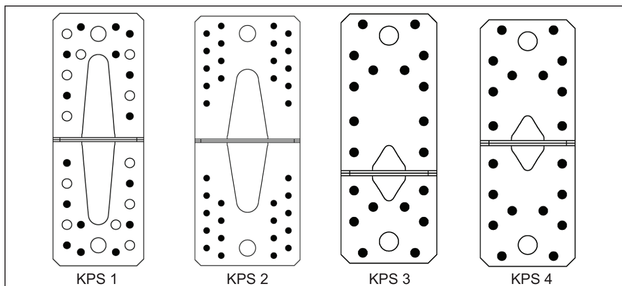
Figure 83 Type KPS
