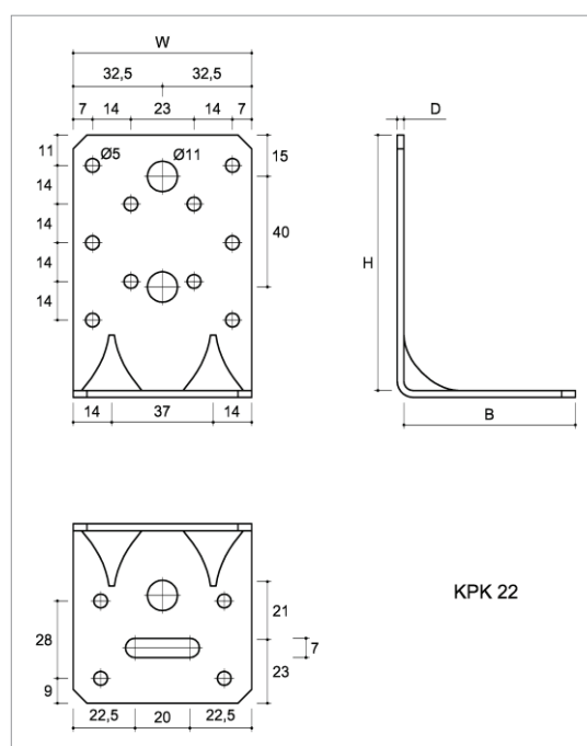
Figure 20 Type KPK 22
