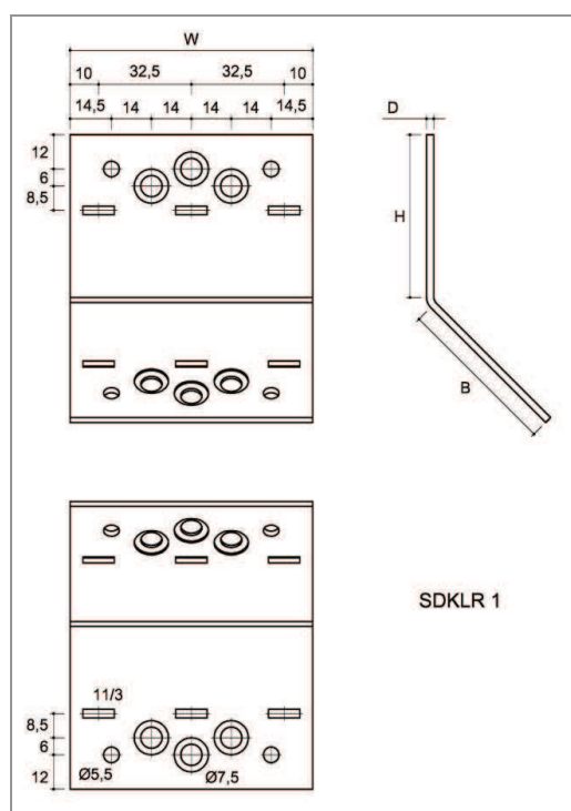
Figure 42 Type SDKLR 1
