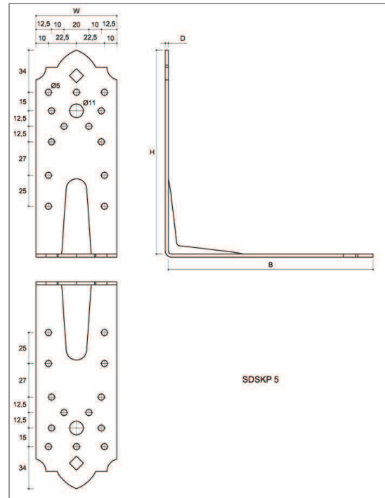
Figure 48 Type SDSKP 5
