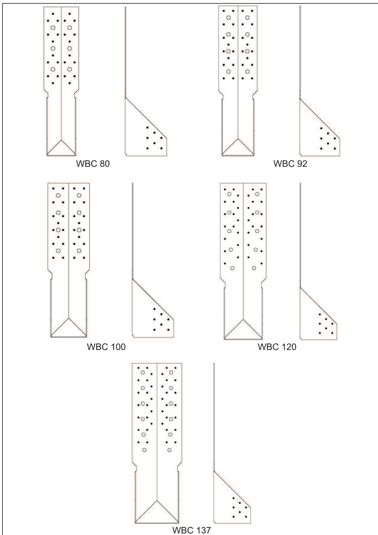
Figure 93 Type WBC
