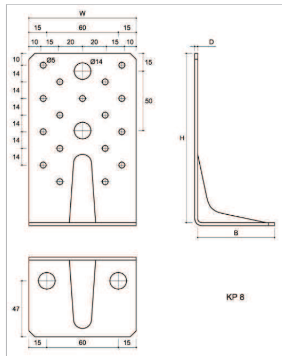
Figure 11 Type KP 8
