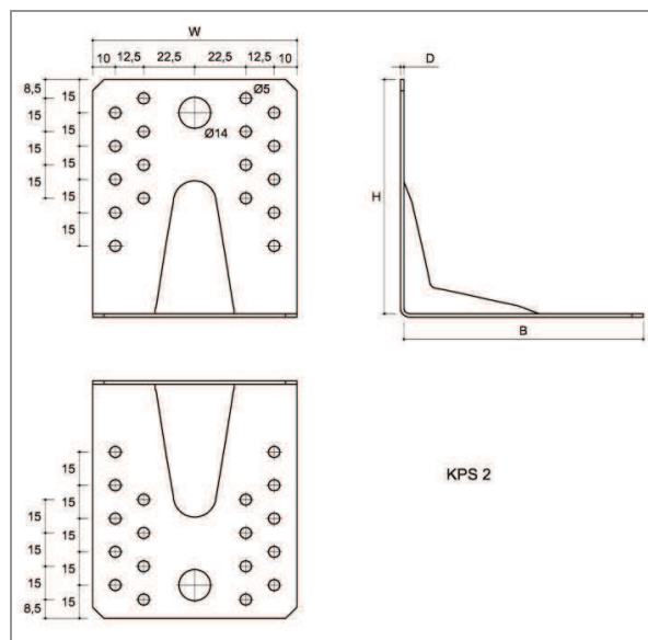
Figure 13 Type KPS 2
