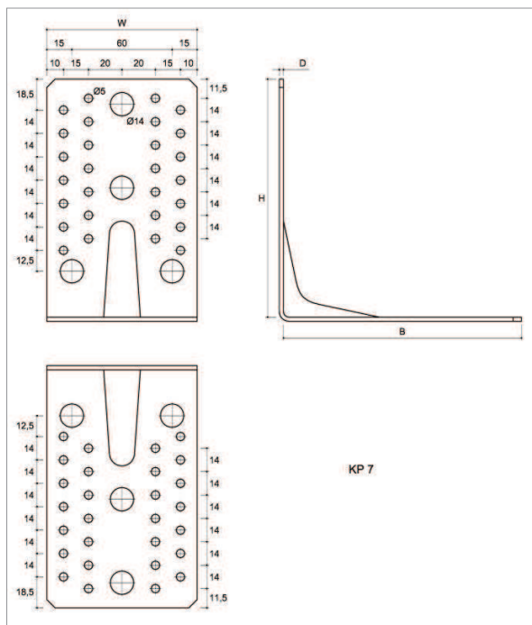
Figure 10 Type KP 7
