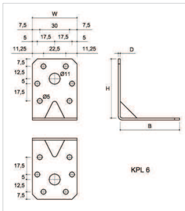
Figure 27 Type KPL 6
