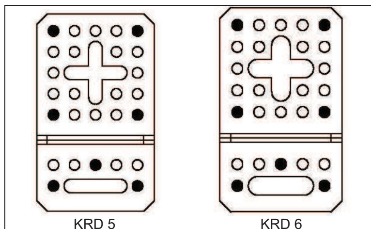
Figure 87 Type KRD
