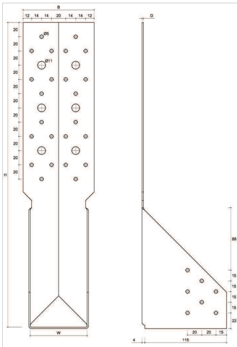
Figure 38 Type WBC 80
