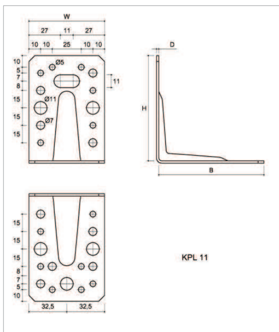
Figure 28 Type KPL 11
