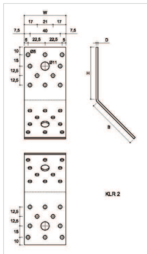
Figure 5 Type KLR 2
