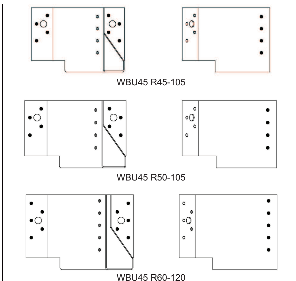
Figure 92 Type WBU
