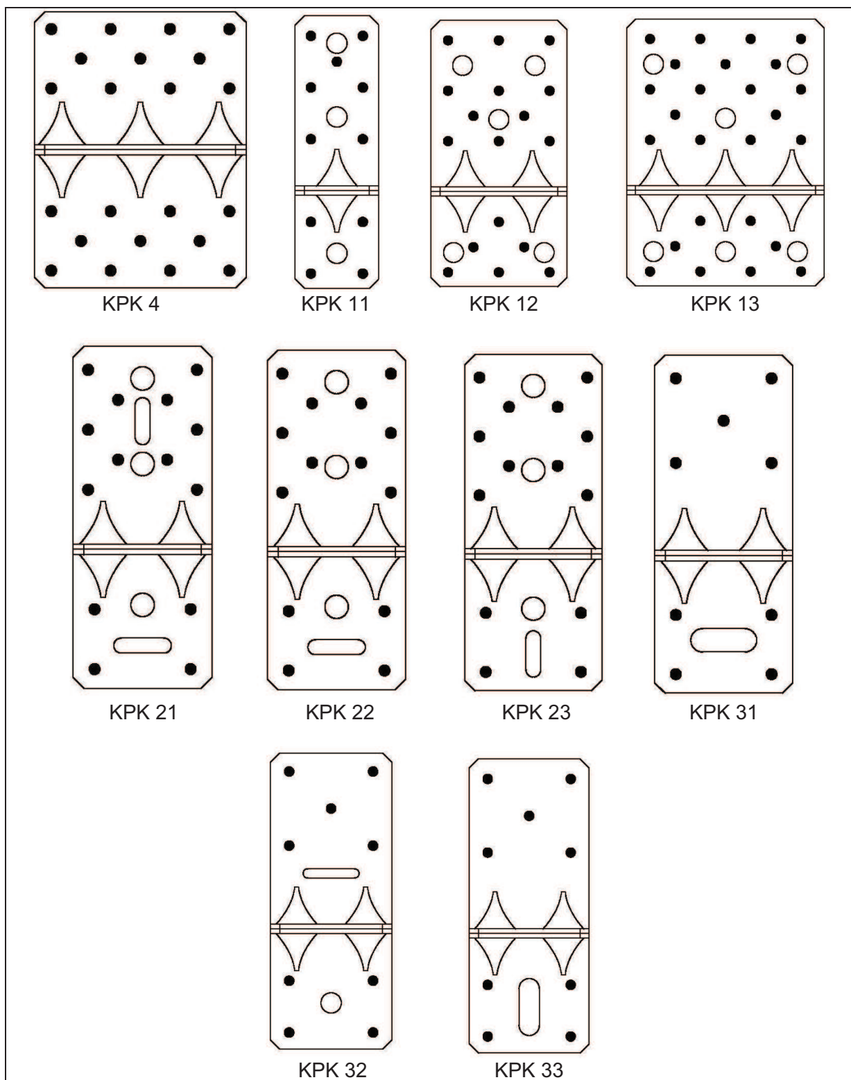
Figure 84 Type KPK
