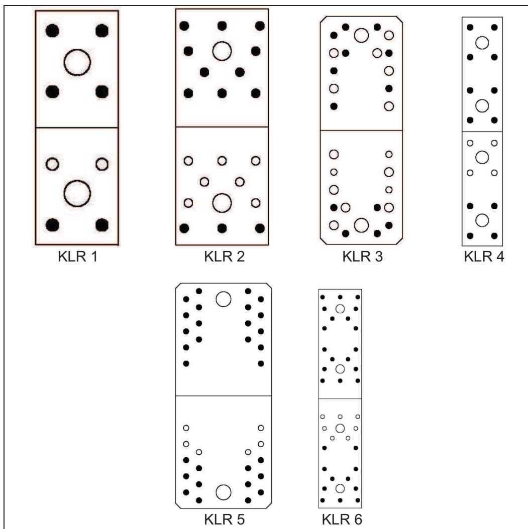
Figure 81 Type KLR
