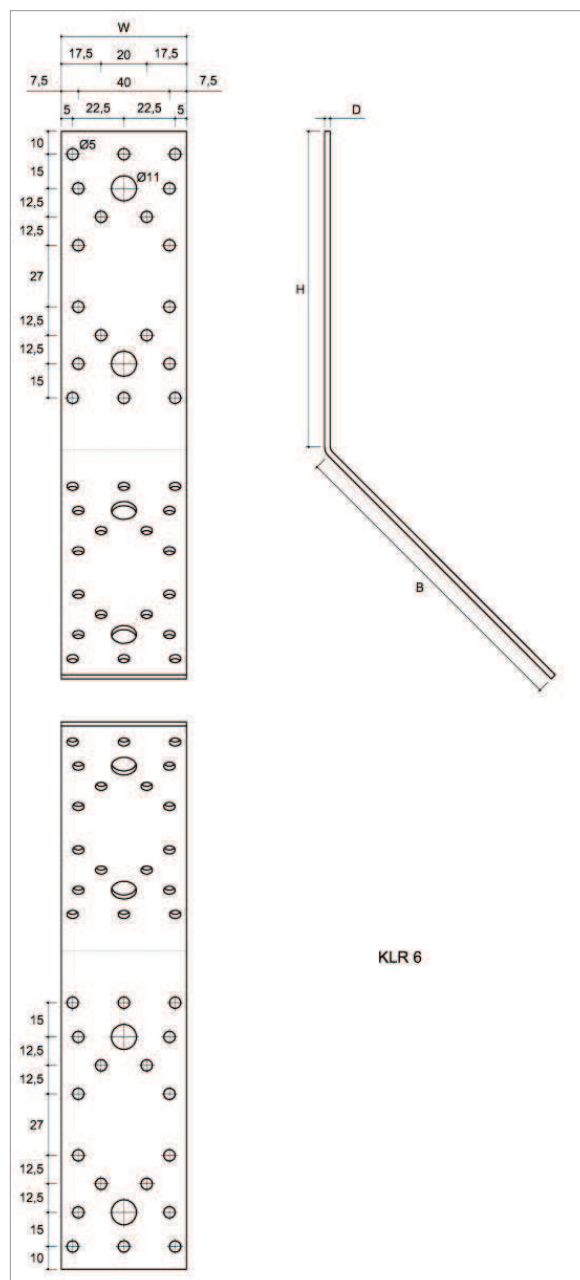
Figure 9 Type KLR 6
