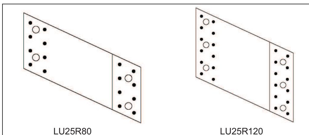
Figure 89 Type LU
