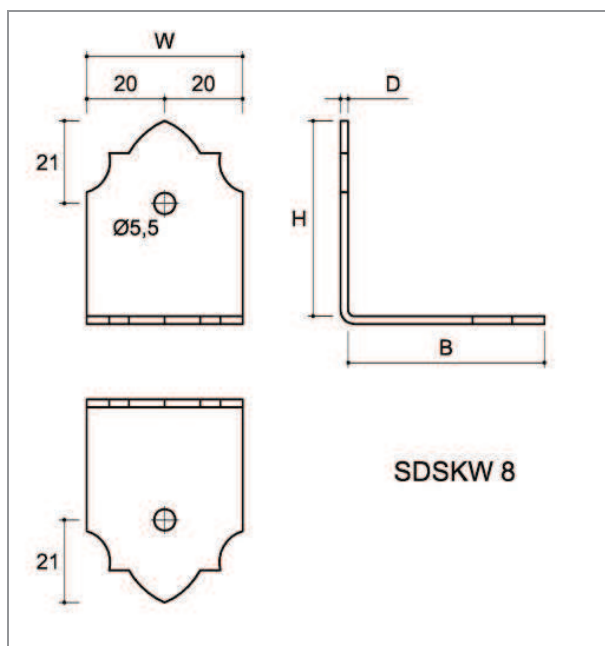
Figure 50 Type SDSKW 8
