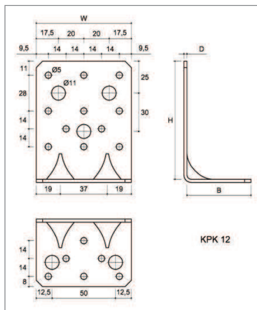
Figure 18 Type KPK 12
