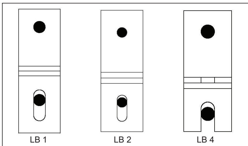
Figure 88 Type LB
